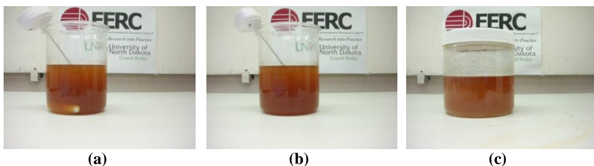
Figure 7-15. Crude jatropha oil – biocrude blend, mixed and held at 75°F. (a) immediately after five minutes of stirring, (b) 25 minutes after stirring, (c) 560 days after stirring.
