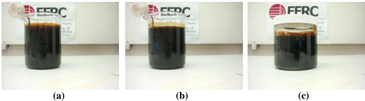
Figure 7-26. Lo-pour fuel oil – crude jatropha oil blend, mixed and held at 170°F. (a) immediately after five minutes of stirring, (b) 25 minutes after stirring, (c) four days after stirring.
