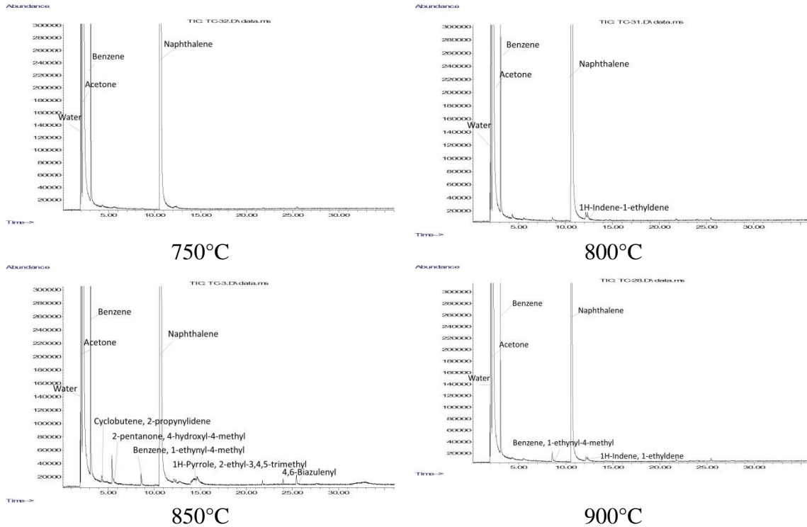
Figure 4-7. GC-MS results for no catalyst runs using syngas blend.
