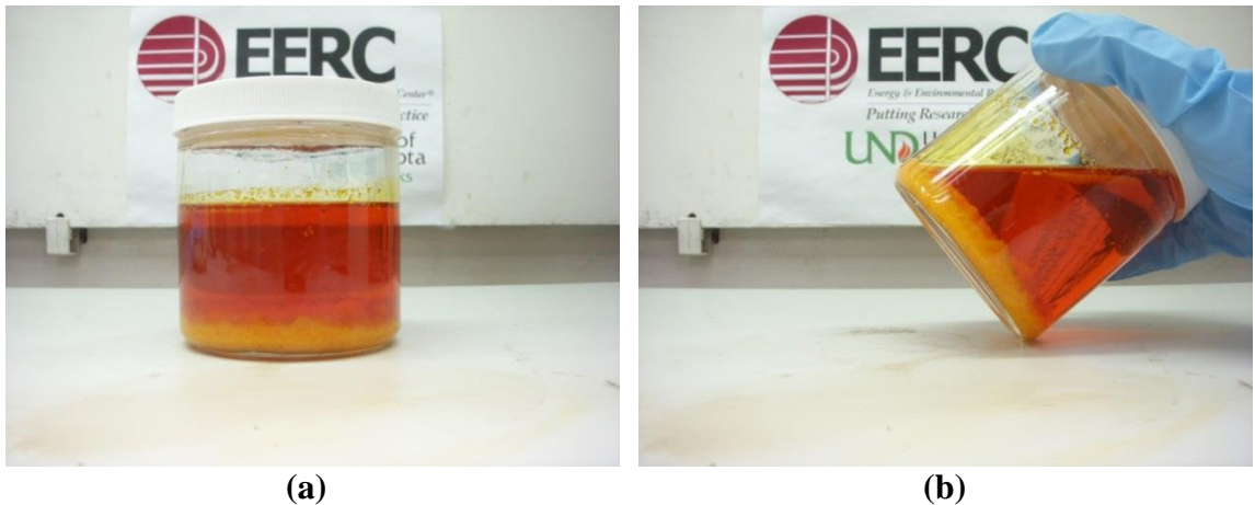
Figure 7-71. Crude palm oil – ultra-low sulfur diesel blend, cooled from 170°F to 75°F. (a) shows the blend sitting flat, and (b) shows the blend tilted at an angle.
