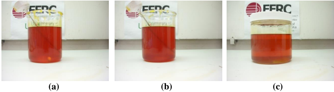
Figure 7-33. Crude palm oil – ultra-low sulfur diesel blend, mixed and held at 170°F. (a) immediately after five minutes of stirring, (b) 25 minutes after stirring, (c) six days after stirring.
