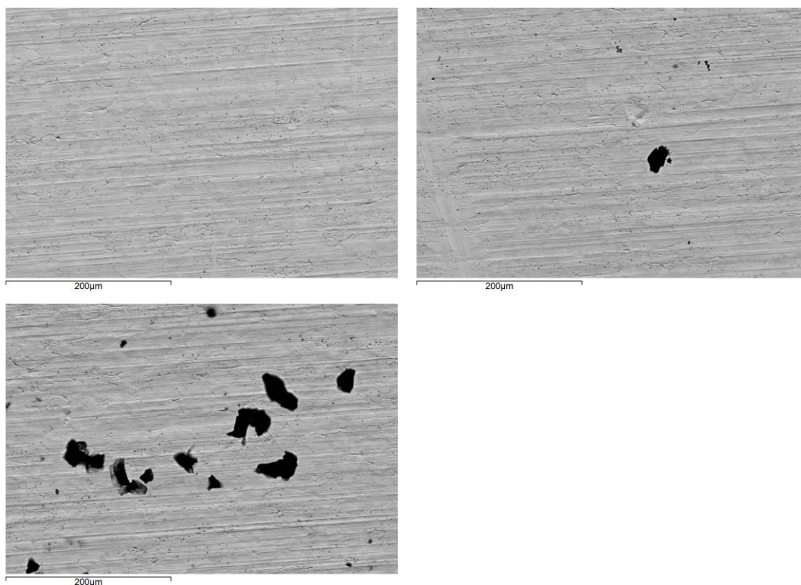
Figure 7-139. Backscatter electron images of 410 stainless steel after 2340 hours of exposure to hi-pour fuel oil.
