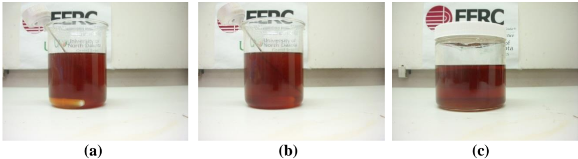
Figure 7-34. Crude jatropha oil – biocrude blend, mixed and held at 170°F. (a) immediately after five minutes of stirring, (b) 25 minutes after stirring, (c) six days after stirring.
