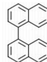
4,4'-binaphthalene
