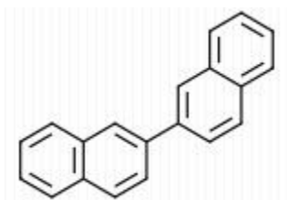
2,2'-binaphthalene
