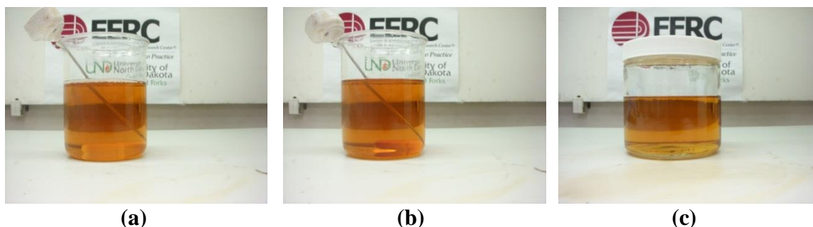
Figure 7-54. Crude jatropha oil – biodiesel blend, mixed and held at 220°F. (a) immediately after five minutes of stirring, (b) 25 minutes after stirring, (c) six days after stirring.
