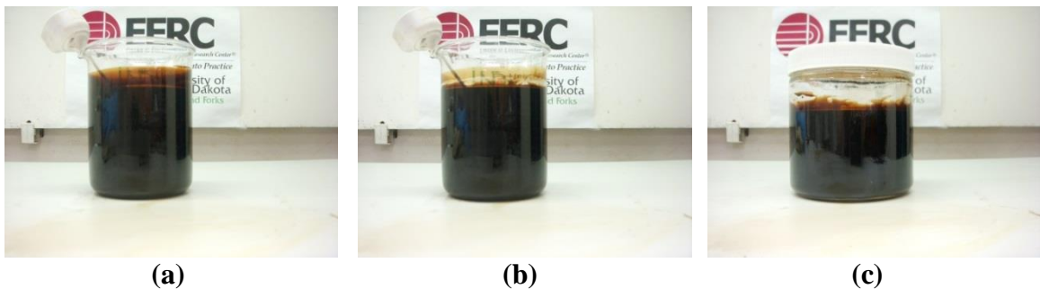
Figure 7-45. Lo-pour fuel oil – crude jatropha oil blend, mixed and held at 220°F. (a) immediately after five minutes of stirring, (b) 25 minutes after stirring, (c) three days after stirring.
