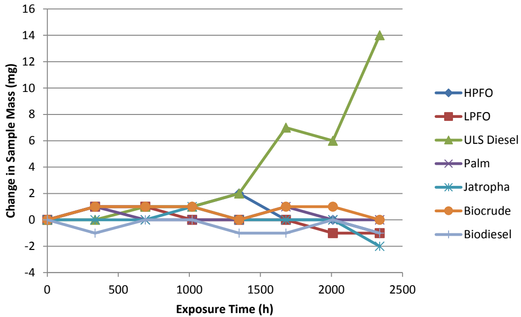
Figure 7-136. Changes in mass of 410 stainless steel samples during testing period.
