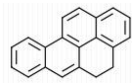
Benzo[a]pyrene, 4,5-dihydro
